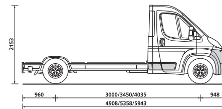
Plancher Cabine Version 4T
