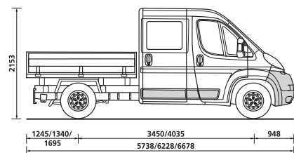
Plateaux Double Cabine
