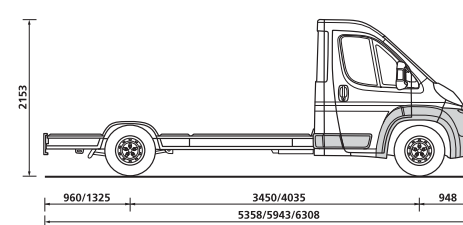
Plancher Cabine Version 4T
