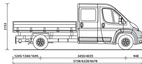
Plateaux Double Cabine Version 4T
